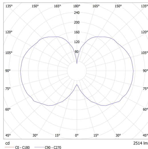
Lucis ZK.L2B.M500 PA MAIA LED / LDC (Polar)
