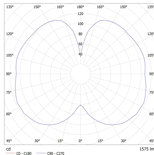
Lucis ZK.L2B.M320 MAIA LED / LDC (Polar)
