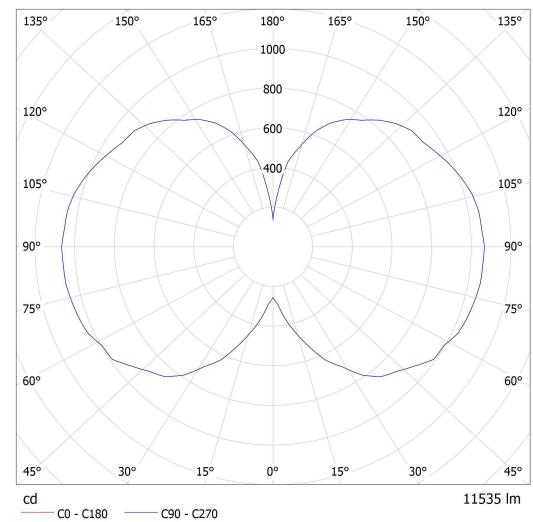
Lucis ZK.L1B.M800 PA MAIA LED / LDC (Polar)
