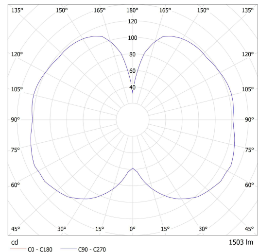
Lucis ZK.L1B.M320 MAIA LED / LDC (Polar)
