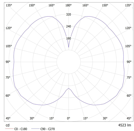
Lucis ZK.L1B.M620 MAIA LED / LDC (Polar)
