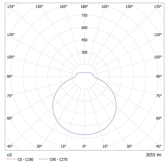
Lucis S44.K4.TEZ4 TENDO LED / LDC (Polar)
