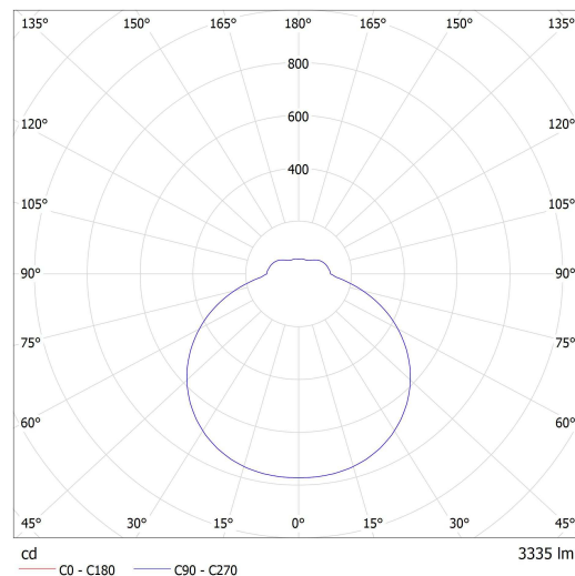
Lucis S33.K1.TEZ3 TENDO LED / LDC (Polar)
