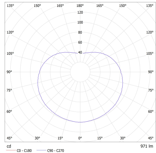
Luminaire: Lucis SR.L2.P1.45M PALA LED Lamps: 1 x LED G6
