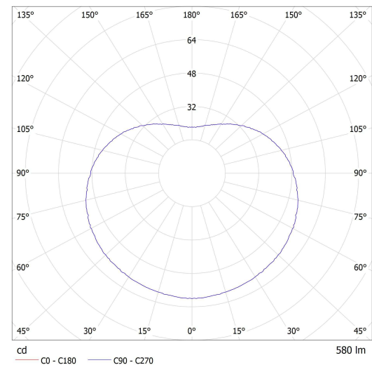
Lucis ZK4.L1.G140.61_pc(4) GEO LED / LDC (Polar)
