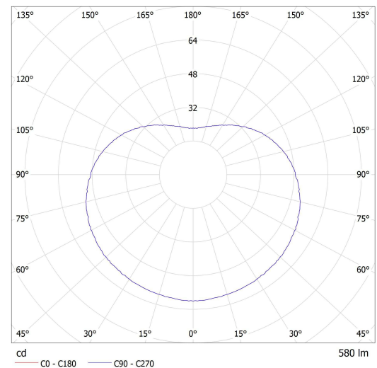
Lucis ZK4.L1.G100.61_pc(4) GEO LED / LDC (Polar)
