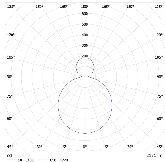
Lucis ZT.K2.R450.X RONDO LED / LDC (Polar)
