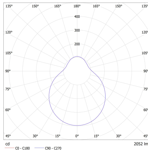
Luminaire: Lucis ZL3.L6.D451.X DAPHNE LED Lamps: 1 x LED G6
