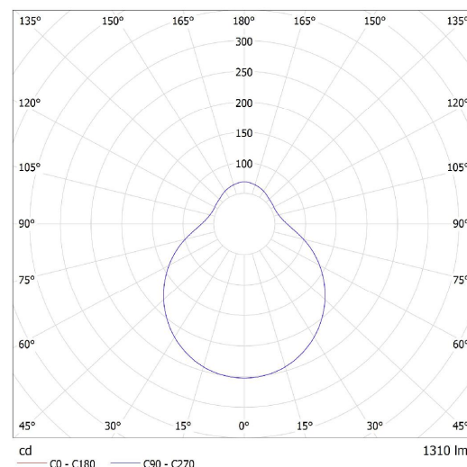
Lucis ZL3.L4.D351.X DAPHNE LED / LDC (Polar)
