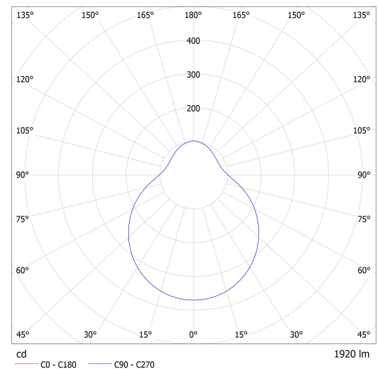
Lucis ZL3.L2.D351.X DAPHNE LED / LDC (Polar)
