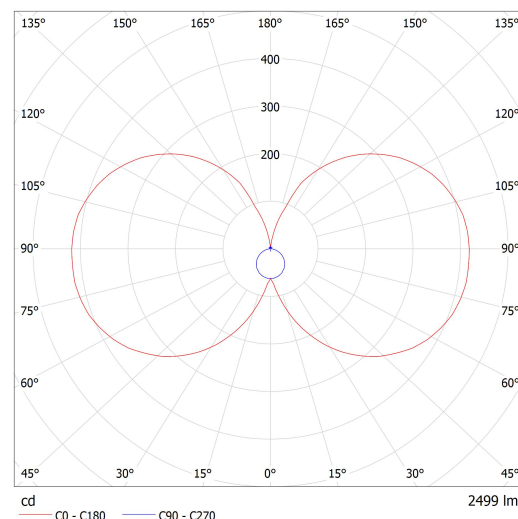
Luminaire: Lucis I2.L2.600.X IZAR METAL LED Lamps: 1 x LED G6
