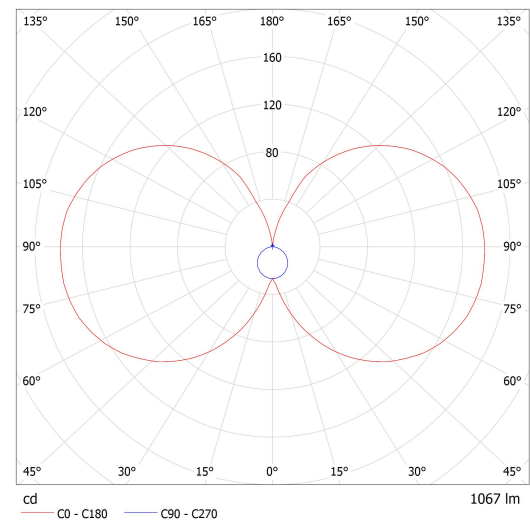
Lucis I2.L1.320.X IZAR METAL LED / LDC (Polar)
