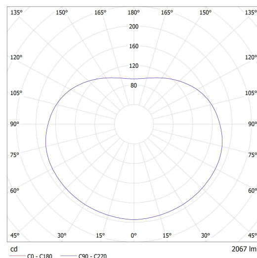
Lucis BS24.L2.350.X POLARIS S LED / LDC (Polar)
