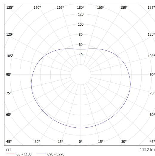
Lucis BS19.L1.280.X POLARIS S LED / LDC (Polar)
