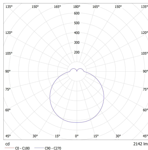
Lucis BS34.K4.N34.X NOMIA LED / LDC (Polar)
