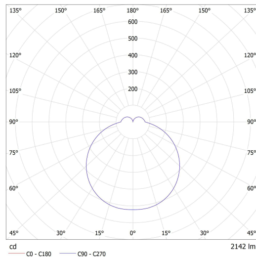
Luminaire: Lucis BS34.K4.N34.X NOMIA LED Lamps: 1 x LED G5
