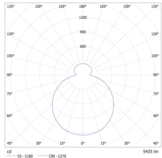
Lucis ZL3.K2.Z600 ZERO LED / LDC (Polar)
