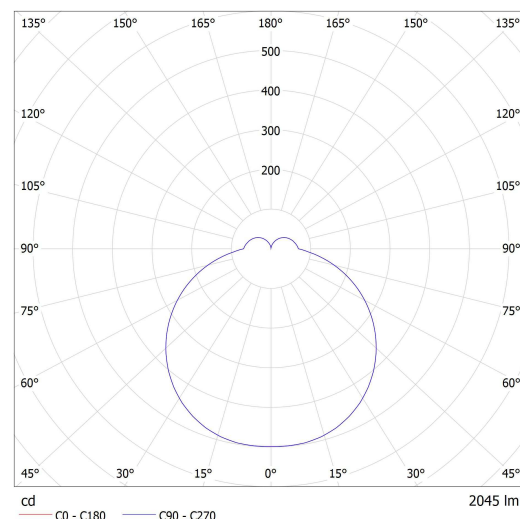
Luminaire: Lucis BS34.K3.N34.X NOMIA LED Lamps: 1 x LED G5
