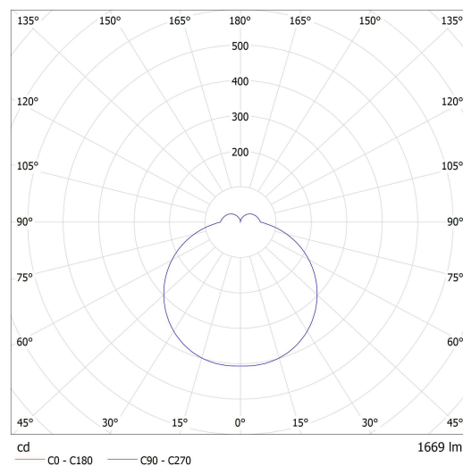
Lucis BS24.K2.N24.X NOMIA LED / LDC (Polar)
