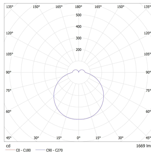
Luminaire: Lucis BS24.K2.N24.X NOMIA LED Lamps: 1 x LED G5
