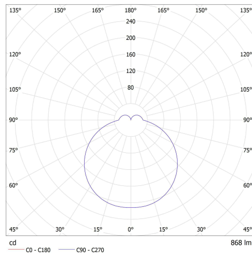
Lucis BS14.K2.N14.X NOMIA LED / LDC (Polar)
