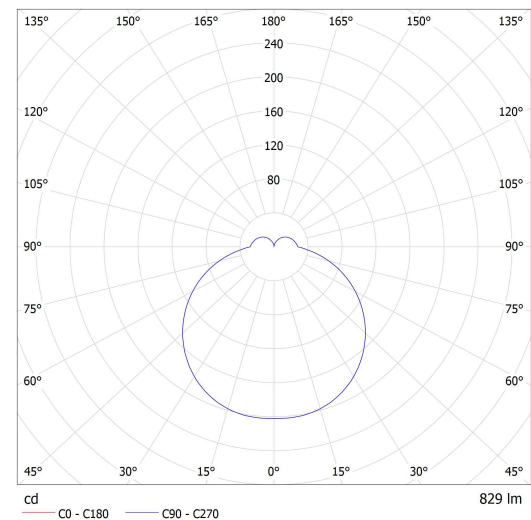
Lucis BS14.K1.N14.X NOMIA LED / LDC (Polar)
