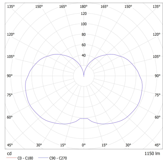
Luminaire: Lucis ZT.L1.R19.X RETRO LED Lamps: 1 x LED G6
