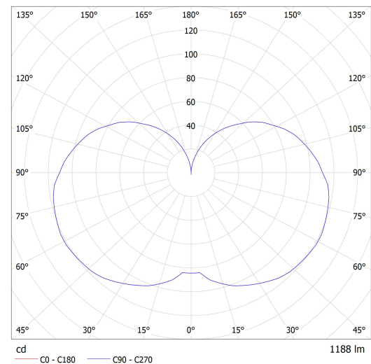
Lucis ZT.L1.R19.X RETRO LED / LDC (Polar)
