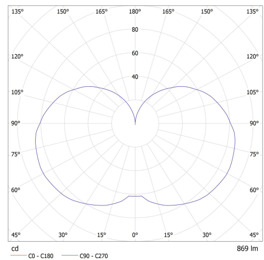
Luminaire: Lucis ZT.L1.R19.X RETRO LED Lamps: 1 x LED G5
