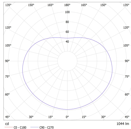
Lucis ZTR.L2.200.X POLARIS ZTR LED / LDC (Polar)
