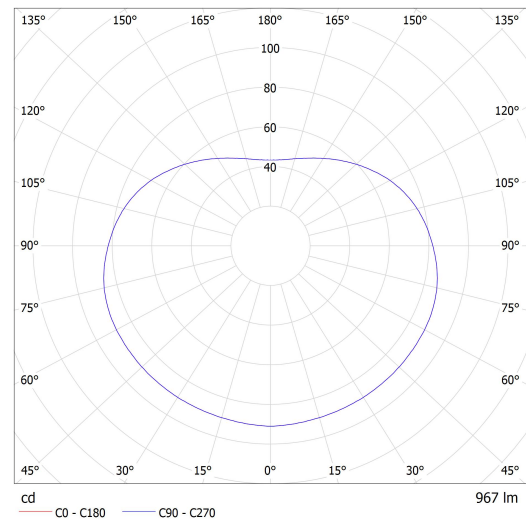
Luminaire: Lucis ZTR.L1.200.X POLARIS ZTR LED Lamps: 1 x LED G6
