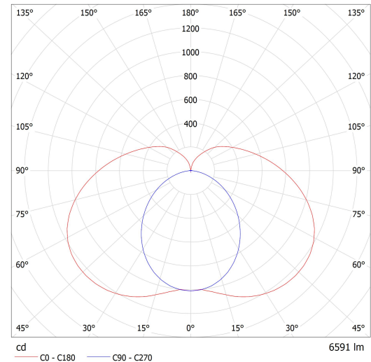
Luminaire: Lucis ZT.AU1.L2.1500.X AULA LED Lamps: 1 x LED G6
