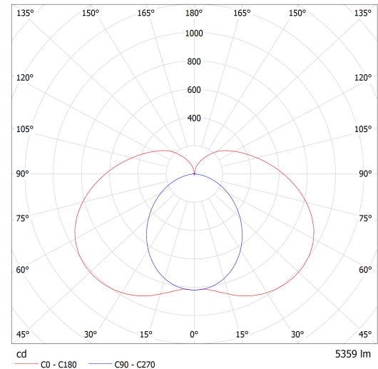
Luminaire: Lucis ZT.AU1.L1.1200.X AULA LED Lamps: 1 x LED G6
