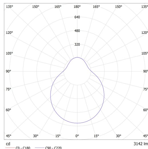
Luminaire: Lucis ZT.L6.D550.X DAPHNE LED Lamps: 1 x LED G6
