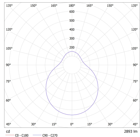
Luminaire: Lucis PS13.L5.D550 DAPHNE LED Lamps: 1 x LED G6
