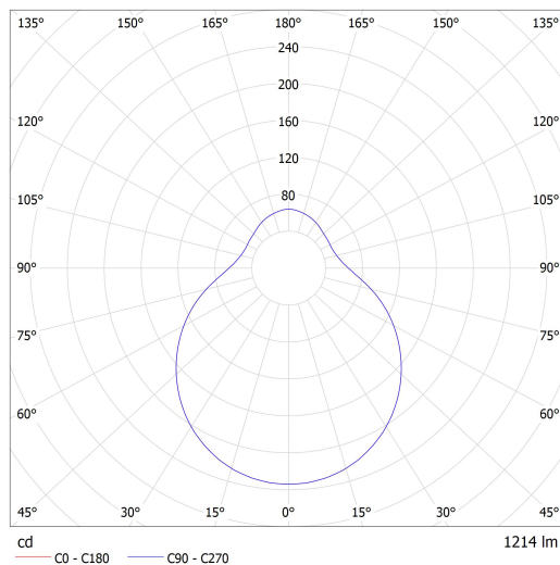
Luminaire: Lucis PS13.L3.D350 DAPHNE LED Lamps: 1 x LED G6
