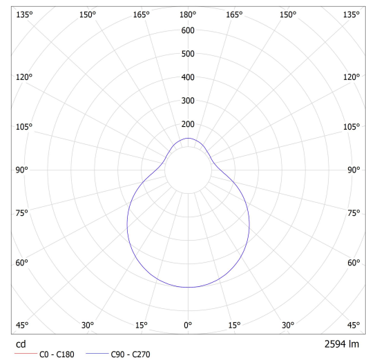
Luminaire: Lucis S34.L6.D450 DAPHNE LED Lamps: 1 x LED G6
