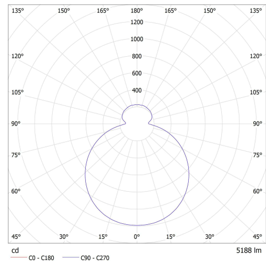
Lucis ZL3.K1.Z600 ZERO LED / LDC (Polar)
