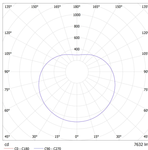
Lucis ZT.P3.600.X POLARIS ZT LED / LDC (Polar)
