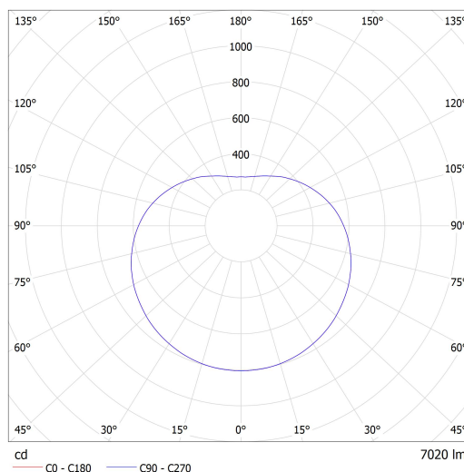
Luminaire: Lucis ZT.P4.500.X POLARIS ZT LED Lamps: 1 x LED G6
