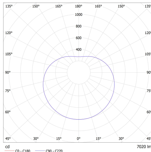
Lucis ZT.P4.500.X POLARIS ZT LED / LDC (Polar)
