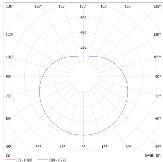
Luminaire: Lucis ZT.P4.400.X POLARIS ZT LED Lamps: 1 x LED G6
