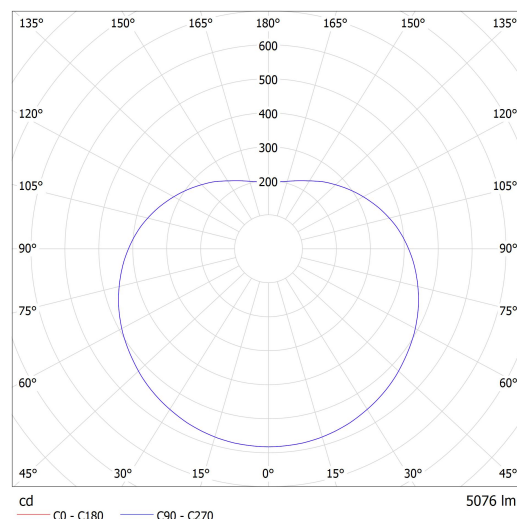
Lucis ZT.P3.400.X POLARIS ZT LED / LDC (Polar)
