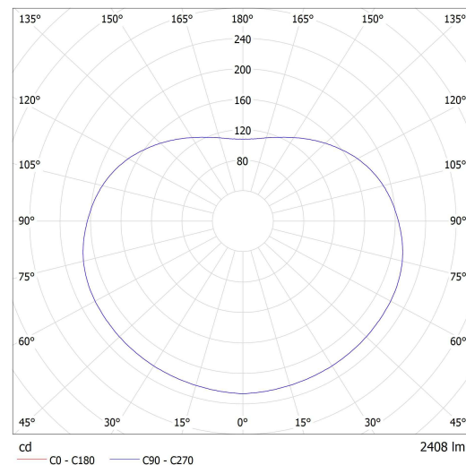
Lucis ZKS.L1.300.X POLARIS ZKS LED / LDC (Polar)
