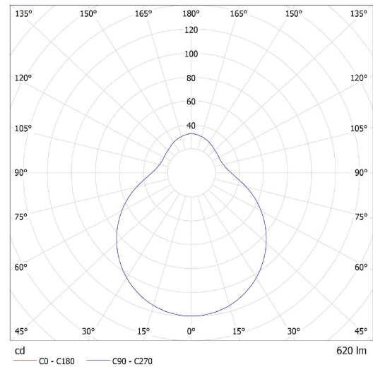
Lucis S19.L14.D280 DAPHNE LED / LDC (Polar)
