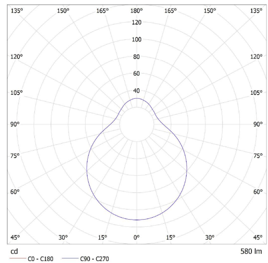
Lucis S19.L13.D280 DAPHNE LED / LDC (Polar)
