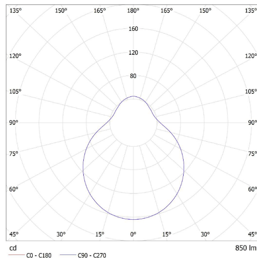
Lucis S19.L2.D280 DAPHNE LED / LDC (Polar)
