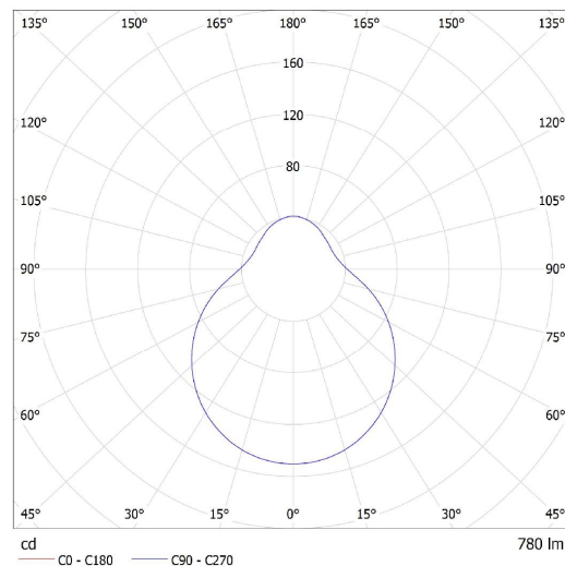
Lucis S19.L1.D280 DAPHNE LED / LDC (Polar)
