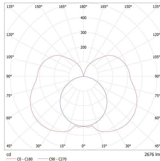
Luminaire: Lucis ZLI3.L4.1200.X IZAR III LED Lamps: 1 x LED G6
