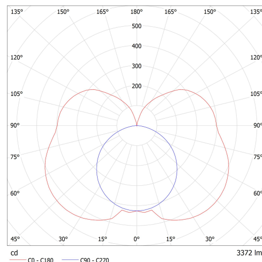
Luminaire: Lucis ZLI3.L3.1500.X IZAR III LED Lamps: 1 x LED G6
