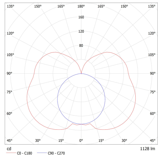
Luminaire: Lucis ZLI3.L3.600.X IZAR III LED Lamps: 1 x LED G6
